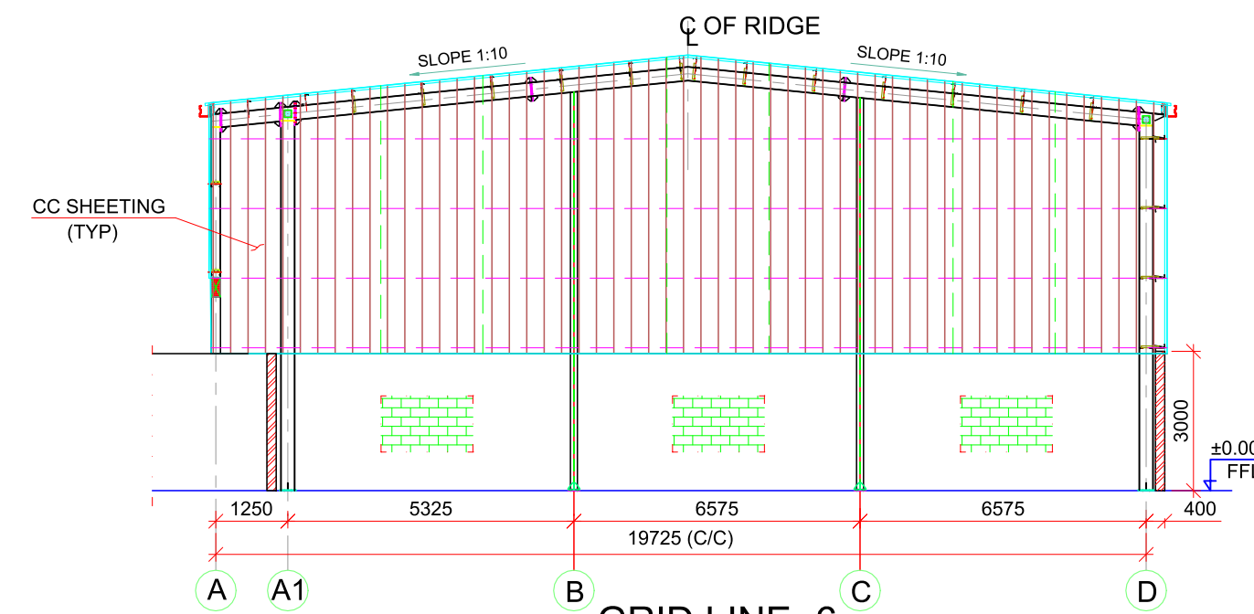
GRID LINE -6
