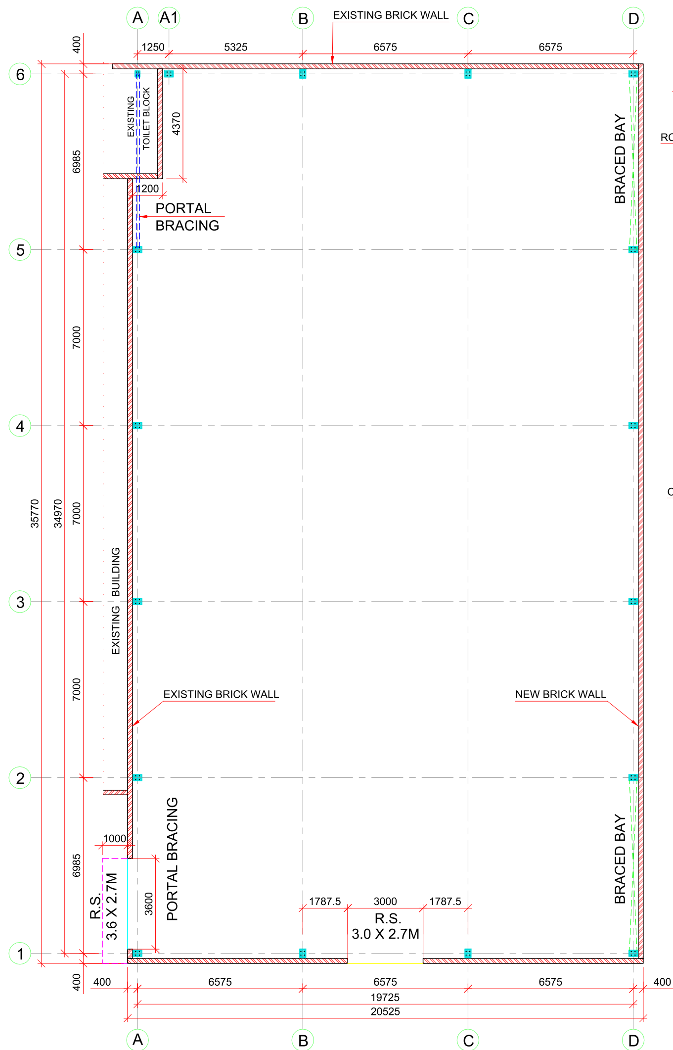
LAYOUT PLAN AT ±0.00 LEVEL
