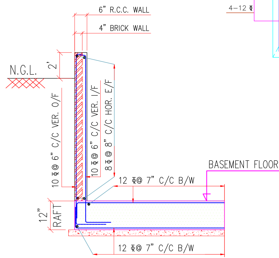
TYP. SECTION 1-1 (FOR R.C.C. WALL & RAFT)
