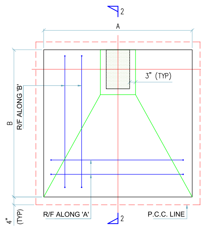
TYP. PLAN OF FOOTING
