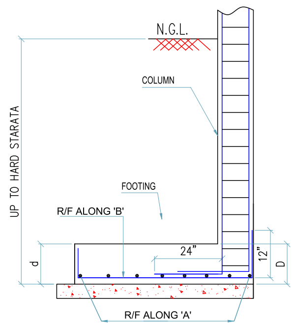
SECTION 2-2 TYP. CROSS SECTIONAL DETAIL OF FOOTING AT CORNER
