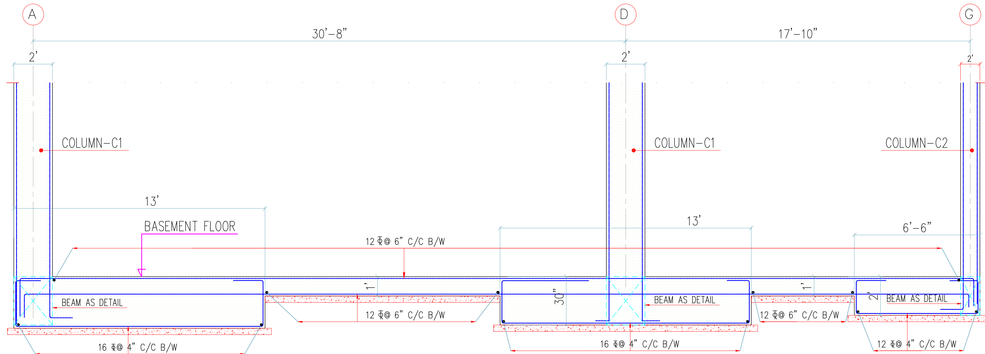
TYP. RAFT & FOOTING SECTION 2-2 (FOR FOOTING & RAFT)
