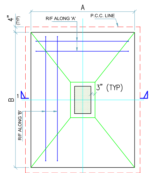
TYP. PLAN OF FOOTING
