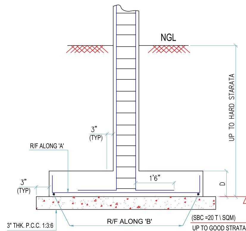
SECTION 1-1
