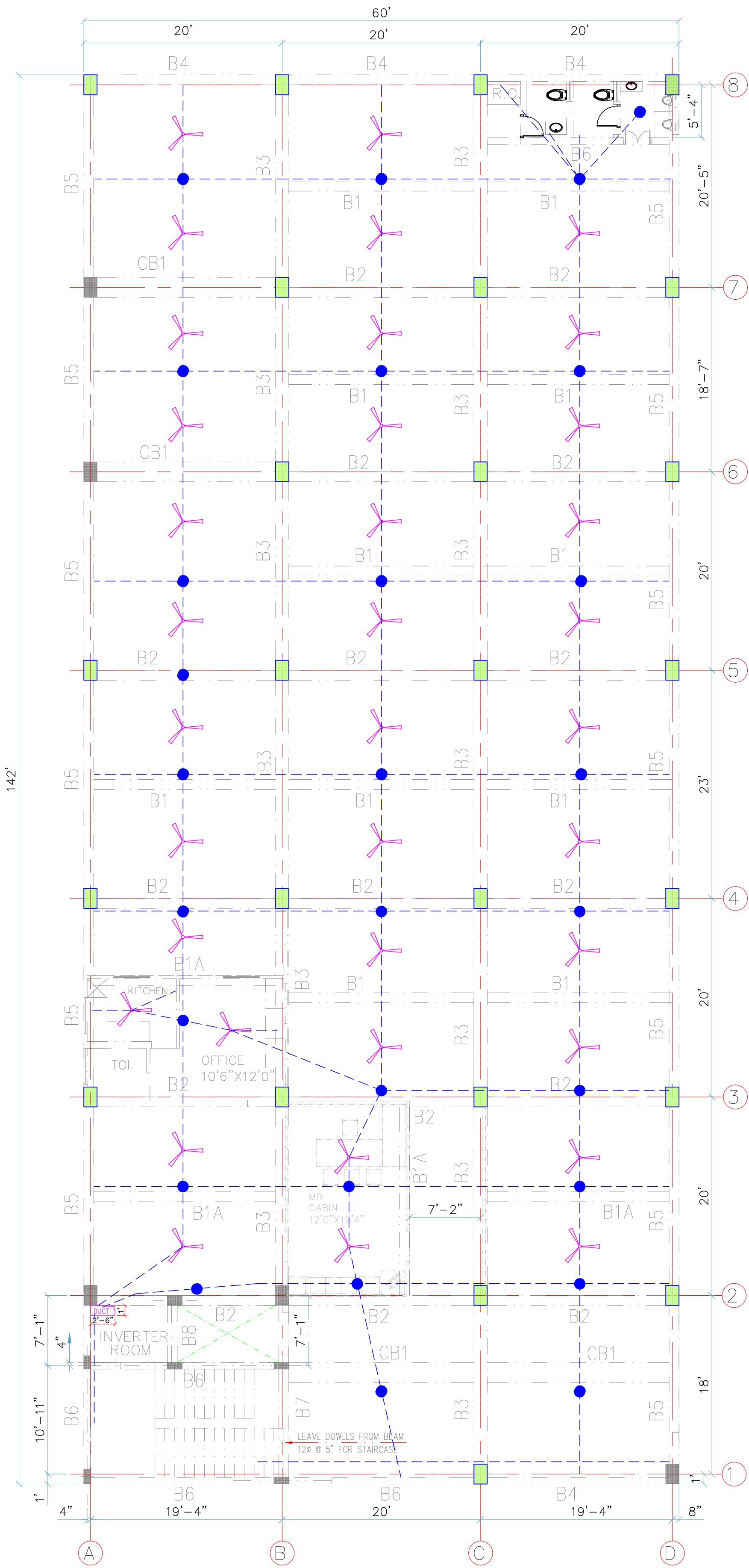
ELECTRIC LINE LAYOUT PLAN AT GROUND FLOOR ROOF
