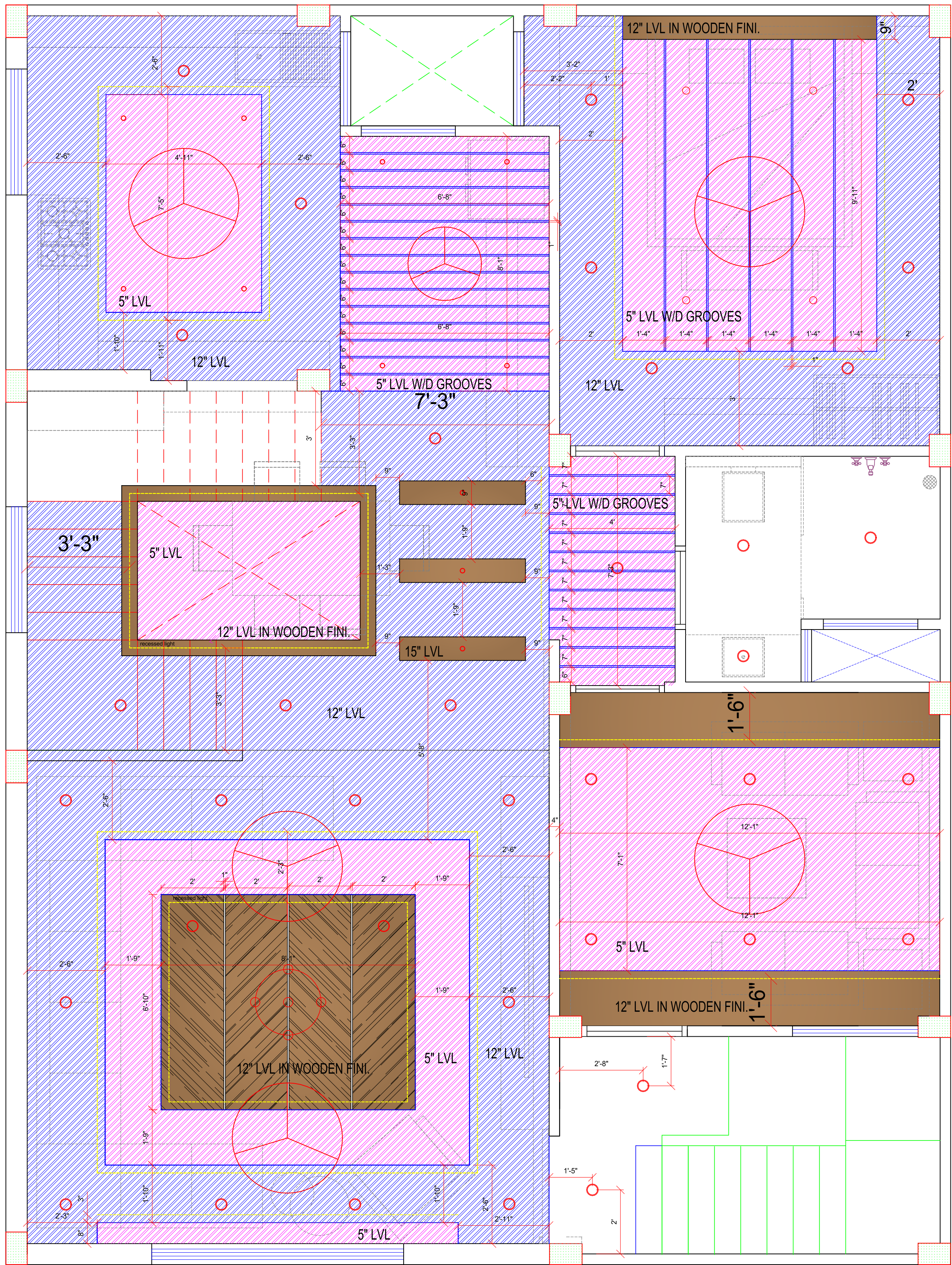
FIRST FLOOR FALSE CEILING W/D ELECTRICAL LAYOUT PLAN
