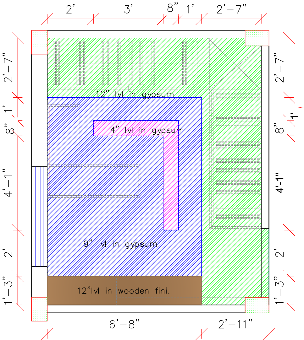
CLOSET CEILING PLAN
