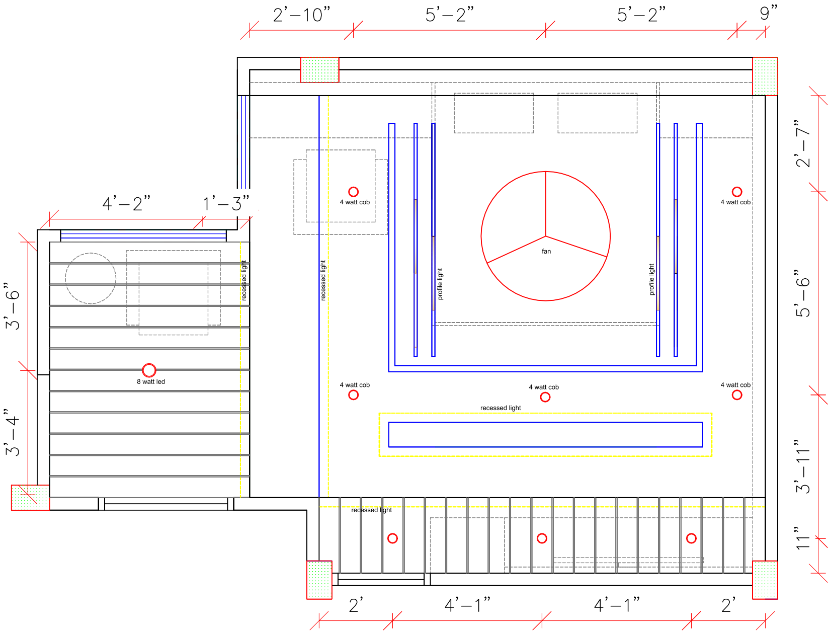
MASTER ROOM ELECTRICAL PLAN
