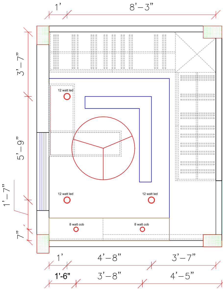
CLOSET ELECTRICAL PLAN
