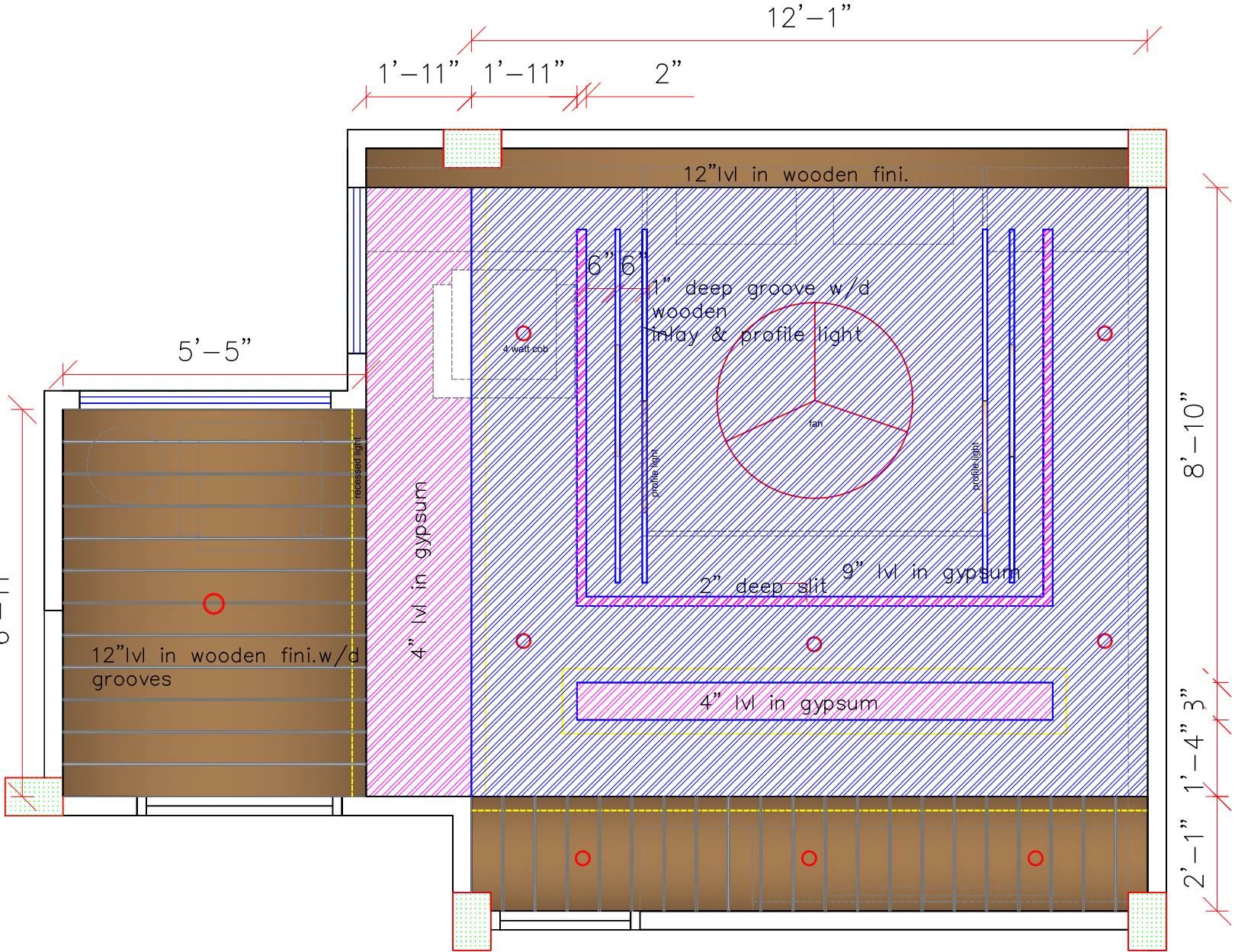
MASTER ROOM CEILING PLAN
