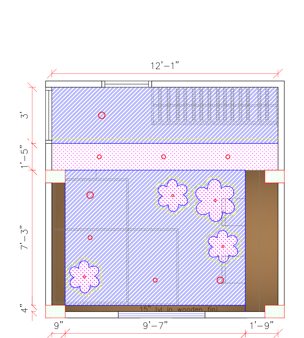
KIDS ROOM CEILING PLAN
