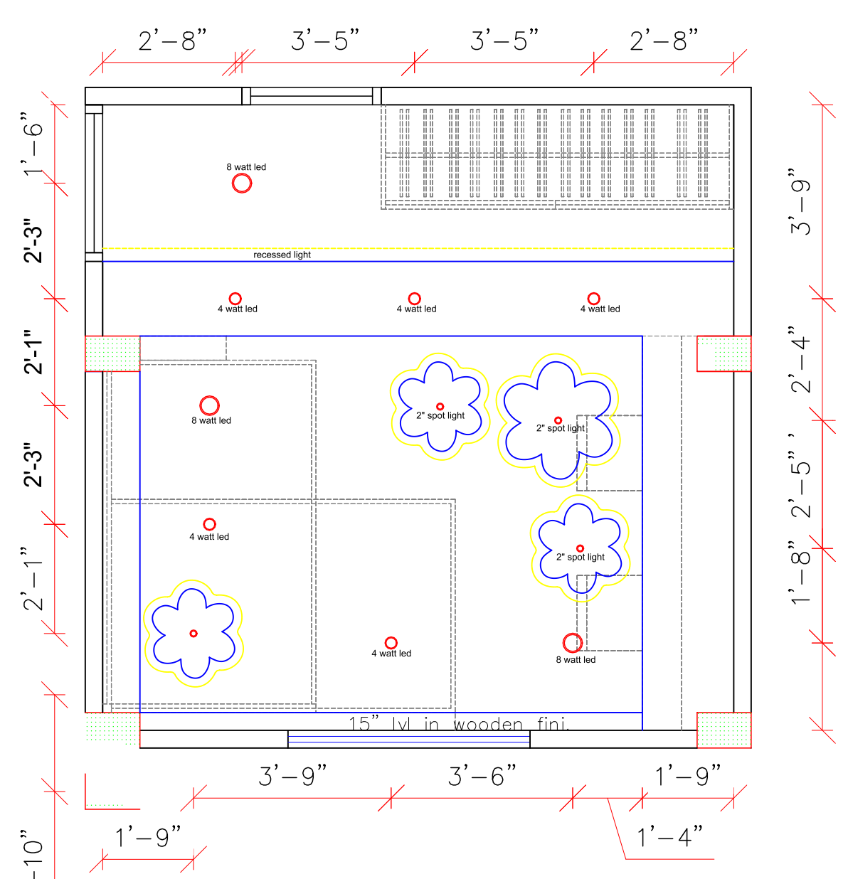
KIDS ROOM ELECTRICAL PLAN
