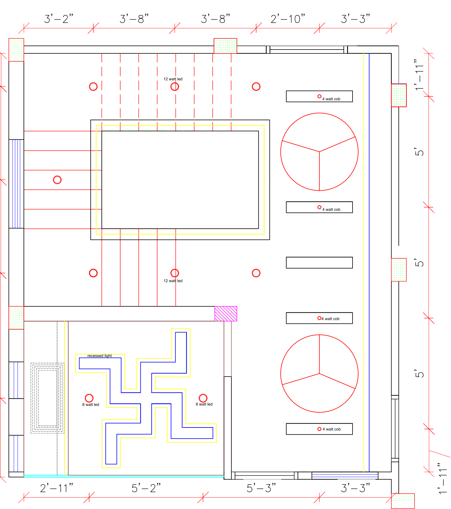
LOUNGE & MANDIR ELECTRICAL PLAN
