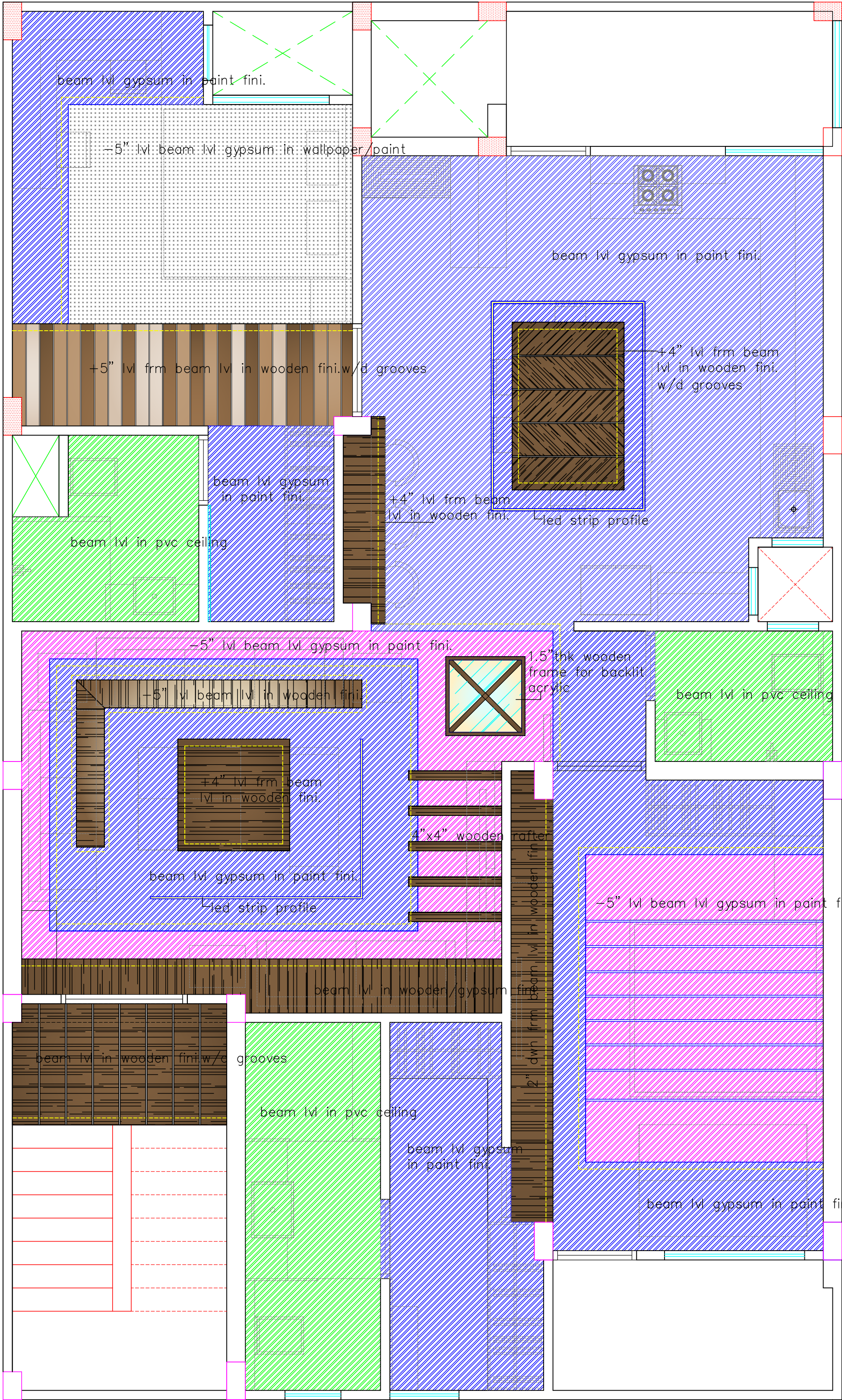
FALSE CEILING PLAN
